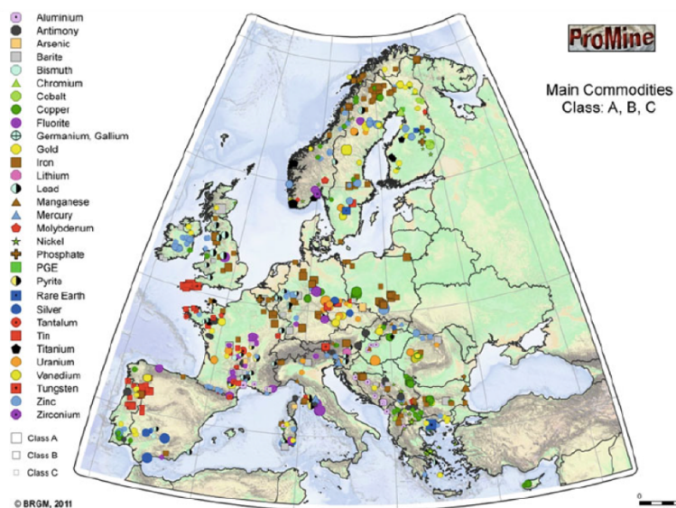
Figure 3. Europe's raw materials potential. Distribution of mineral deposits in Europe (BRGM 2011) and main commodities by mineral belts.
